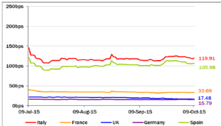
5 Years CDS levels Countries
